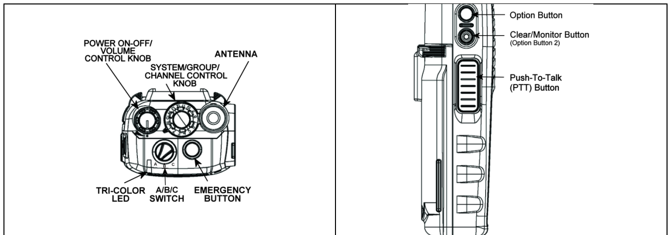
Figure 8-1: Top View
