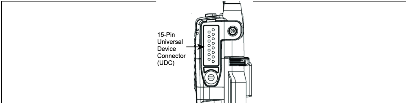
Figure 8-7: XG-75Pe 15-Pin Universal Device Connector
